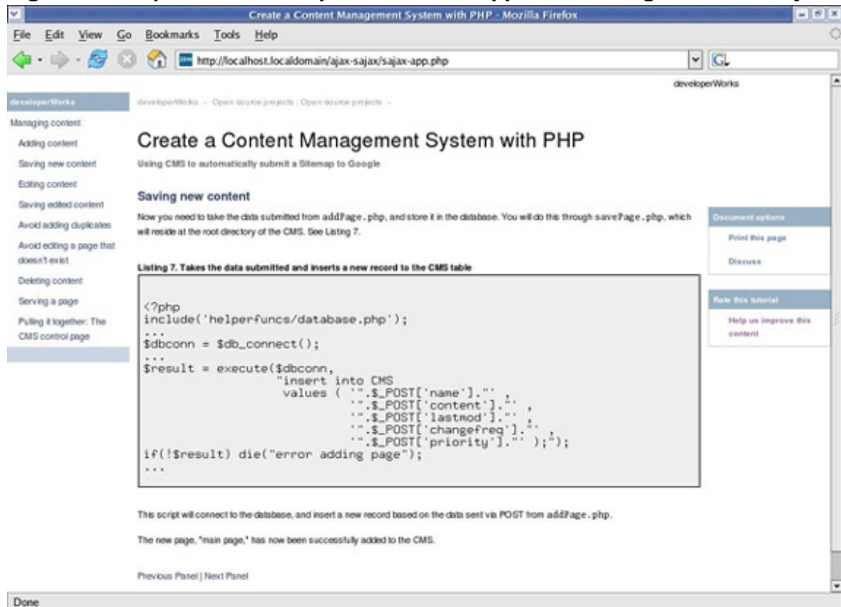
Figure 5. Sample browser output of the PHP application integrated with Sajax
